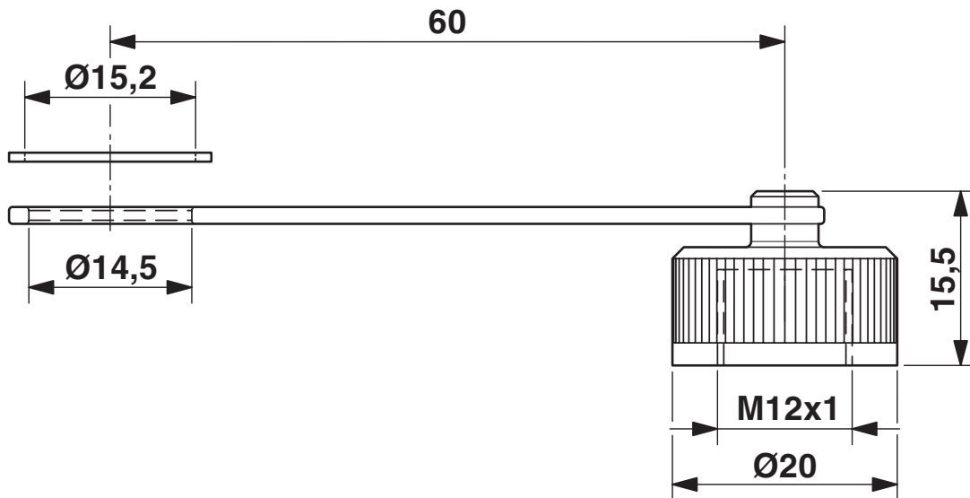
Dimensional drawing
